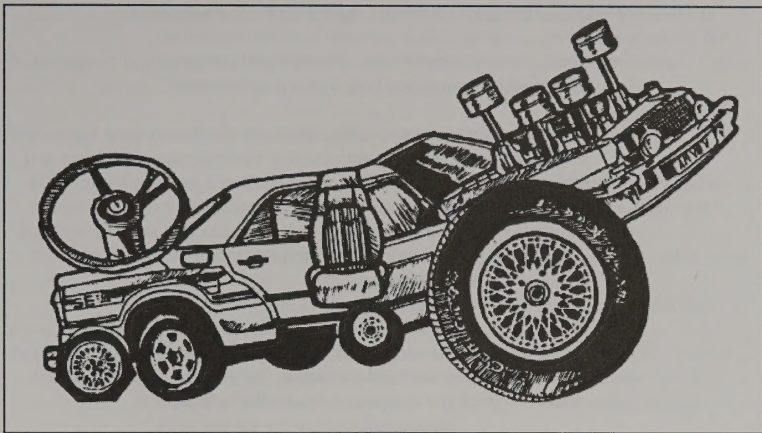
Figure 1. Multidisciplinary.
